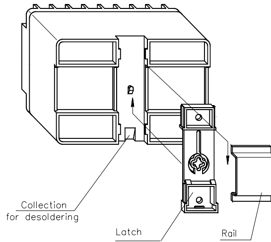
Figure B.1 Mounting of the Rail
